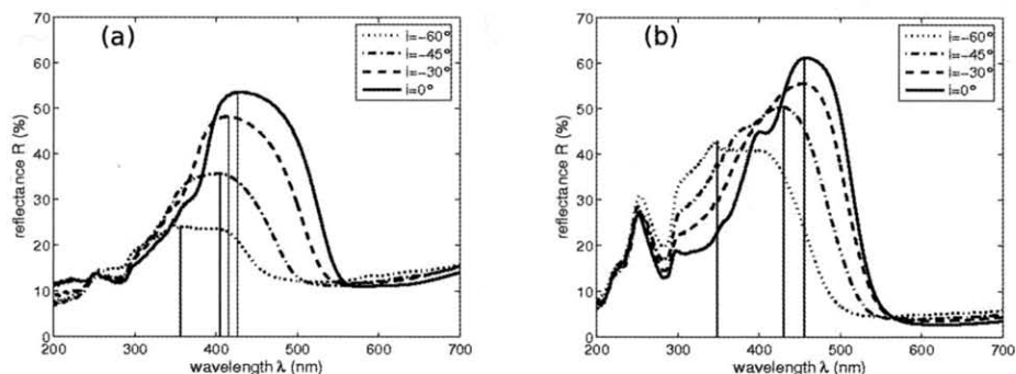
Figure 5: Hemispherical reflectance spectra of (a) Mercedes atnius (HERRICH-SCHÄFFER, 1853) and (b) Morpho rhetenor (CRAMER, 1775) wings at various angles of incidence. Bars indicate the position of the maximum value of reflectance.
