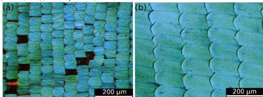
Figure 2: (a) Mercedes atnius (HERRICH-SCHÄFFER, 1853) and (b) Morpho rhetenor (CRAMER, 1775) scales in hind-wing dorsum under normal incidence; showing transparent M. atnius (H.-S.) cover scales and atrophied M. rhetenor (Cr.) cover scale.
