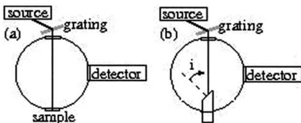
Figure 4: (a) classical mounting and (b) use of substrates with calibrated angles for hemispherical spectroscopy measurement.
