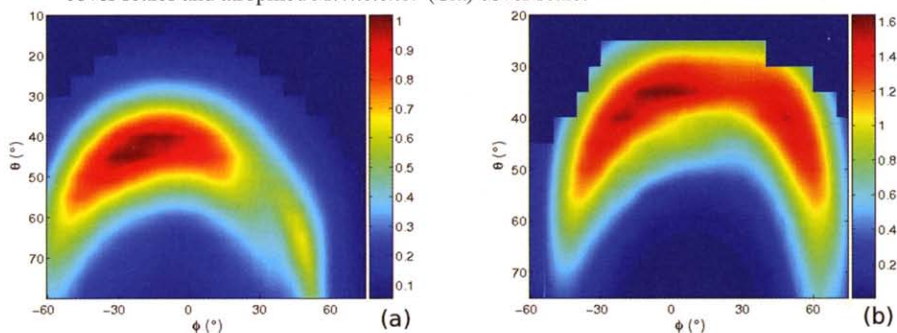
Figure 8: Experimental diffraction maps (BRDF values in s_r^{-1} are in colour scale) for \lambda = 450 nm and (a) \theta_i = 30^\circ for Mercedes atnius (HERRICH-SCHÄFFER, 1853) and (b) \theta_i = 20^\circ for Morpho rhetenor (CRAMER, 1775).
