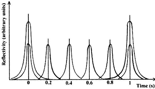
Figure 10: Theoretical signal observed during the flight above the butterfly. This diagram was built copying and translating dispersion graphs of Figure 9.
