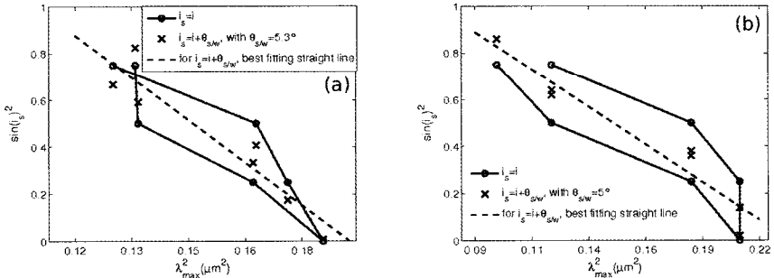
Figure 6: Sine square of the incidence angle versus the square of the wavelength of the reflection maximum for (a) Mercedes atnius (HERRICH-SCHÄFFER, 1853) and (b) Morpho rhetenor (CRAMER, 1775).
