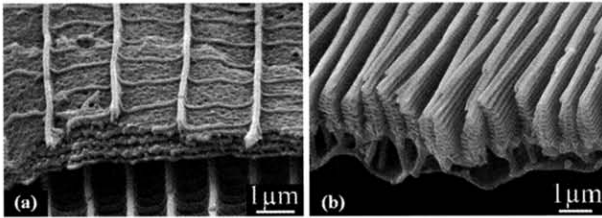
Figure 3: (a) Mercedes atnius (HERRICH-SCHÄFFER, 1853) cover scale and (b) Morpho rhetenor (CRA-MER, 1775) ground scale; SEM images.
